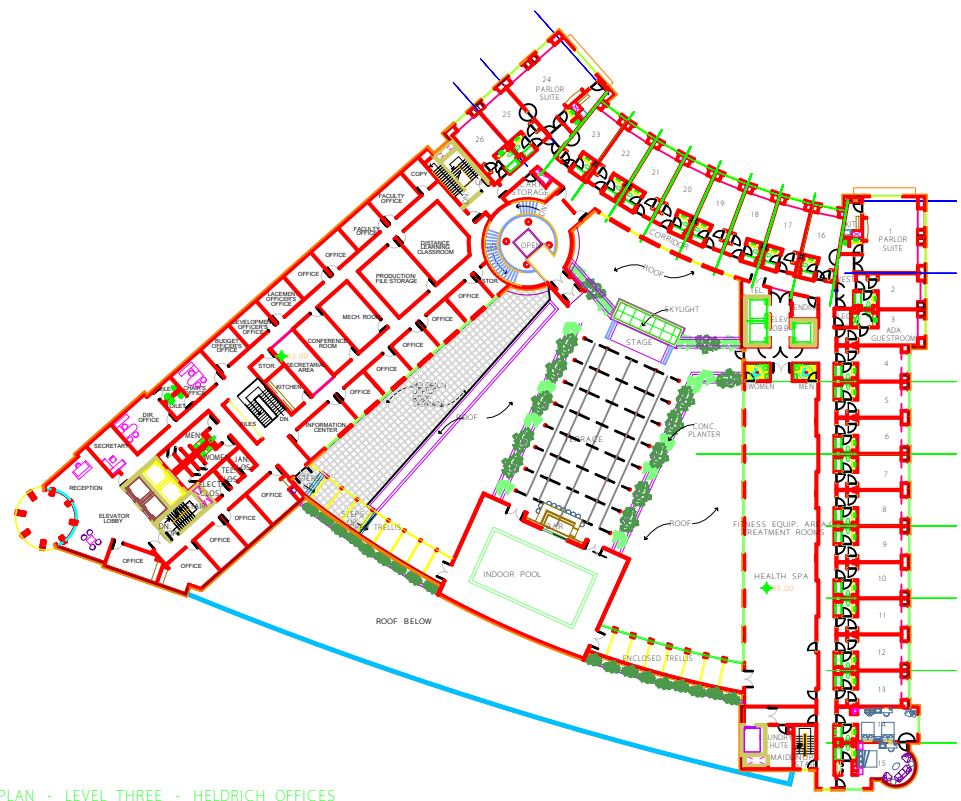
PLAN - LEVEL THREE - HELDRICH OFFICES SCALE: 1/16"=1'-0"
